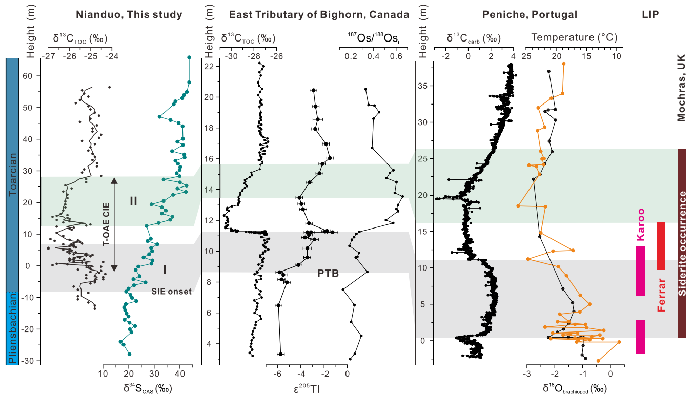
Fig. 6. Multiple early Toarcian geochemical records illustrating the relationship between different environmental perturbations. For Nianduo (Tibet), \delta^{13}\text{C}_{\text{TOC}} data are from Han et al. (2018); For East Tributary of Bighorn (Canada), \delta^{13}\text{C}_{\text{TOC}} data are from Them II et al. (2017), \varepsilon^{205}\text{Tl} data (ocean deoxygenation) from Them et al. (2018) and ^{187}\text{Os}/^{188}\text{Os}_i data (continental weathering) from Them et al. (2017); For Peniche (Portugal), \delta^{13}\text{C}_{\text{carb}} data are from Hesselbo et al. (2007) and \delta^{18}\text{O} data (sea-surface temperature) of brachiopods from Suan et al. (2008) and Müller et al. (2020); For Karoo-Ferrar LIP (Large Igneous Province) activity data are from Burgess et al. (2015); Percival et al. (2015); Xu et al. (2018a) and Al-Suwaidi et al. (2022); For Mochras (UK), the stratigraphic position of siderite occurrence is from Xu et al. (2018b). SIE: sulfur-isotope excursion.
