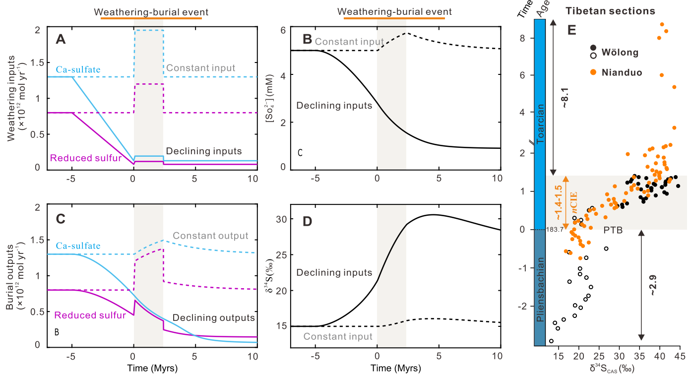
Fig. 5. Long-term sulfur-cycle model for the late Pliensbachian to Toarcian interval. Panels show changes in weathering inputs of Ca-sulfate and reduced sulfur. (A), seawater [\text{SO}_4^{2-}] (B), and paired burial outputs (C) and seawater \delta^{34}\text{S} (D). Dashed lines show default model where weathering inputs of sulfur do not change, and solid lines show model where weathering inputs decrease and [\text{SO}_4^{2-}] drops below the Ca-sulfate deposition threshold, causing a rise in \delta^{34}\text{S} . Panel E shows the Tibetan \delta^{34}\text{S} data calibrated against the numerical time scale that is determined in the Supplementary material; PTB: Pl-To boundary (~183.7 Ma).
