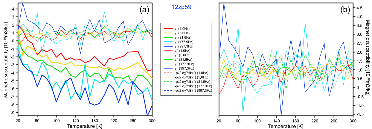
Figure 6. (a) In-phase and quadrature susceptibility at 1.0 Hz, 5.6 Hz, 31.6 Hz, 177.9 Hz, and 997.3 Hz for sample 12ZP59, measured from 20 to 300 K. Strong frequency dependence over the whole temperature range indicates a broad size distribution of nanoparticles. (b) Expanded view of quadrature susceptibilities compared to the derivative of in-phase susceptibility with respect to \ln(f) . Consistency between them implies that quadrature susceptibility originates primarily in a thermal relaxation mechanism.
