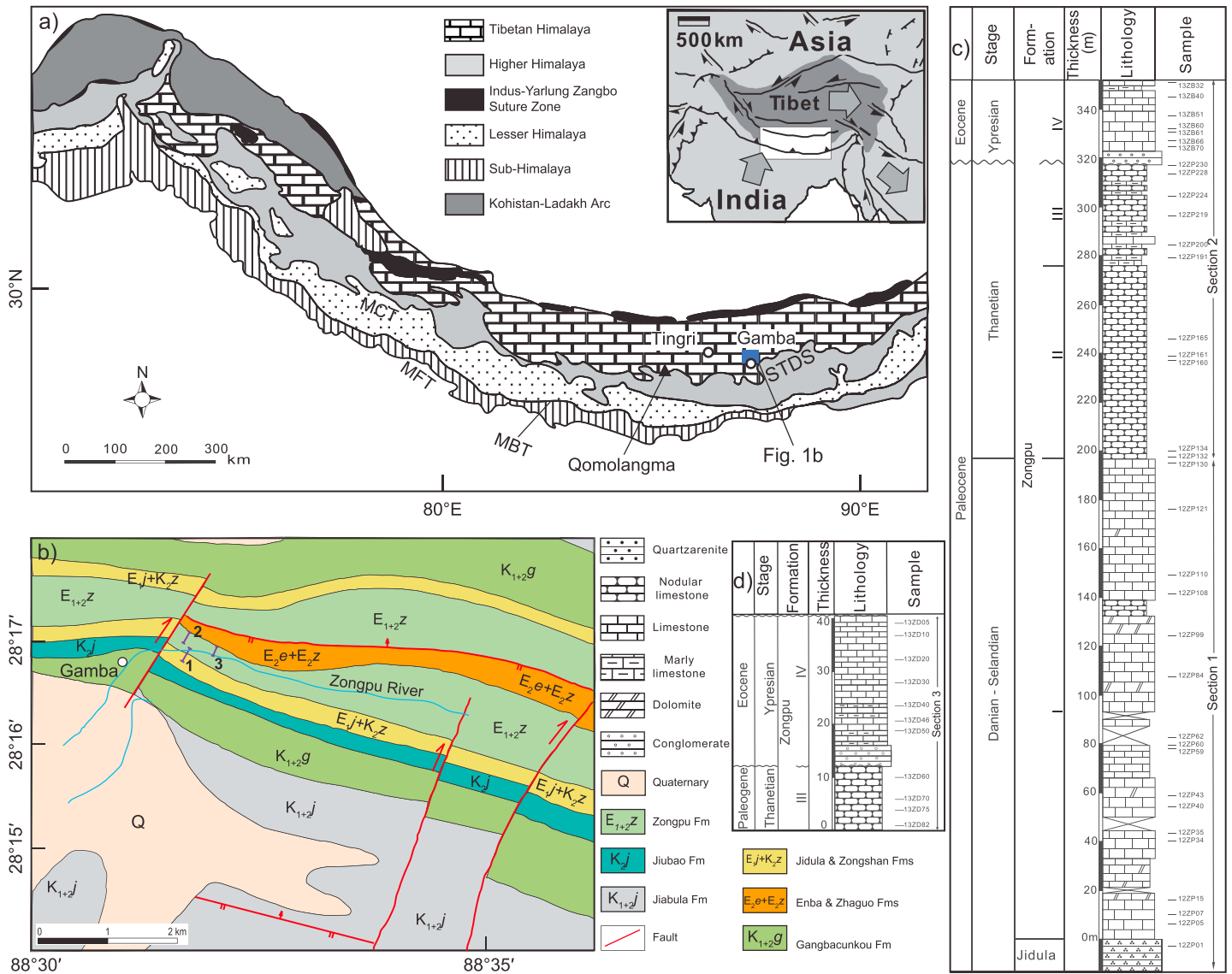
Figure 1. (a) Simplified geologic map of the Himalayas, modified from Li et al. [2015]. MFT: Main Frontal Thrust, MBT: Main Boundary Thrust, MCT: Main Central Thrust, STDS: Southern Tibetan Detachment System. (b) Geologic map of the Gamba area showing the studied stratigraphic sections, modified after Li et al. [2015]. (c and d) Lithostratigraphy of the Zongpu and uppermost Jidula Formations with the sampling localities indicated.
