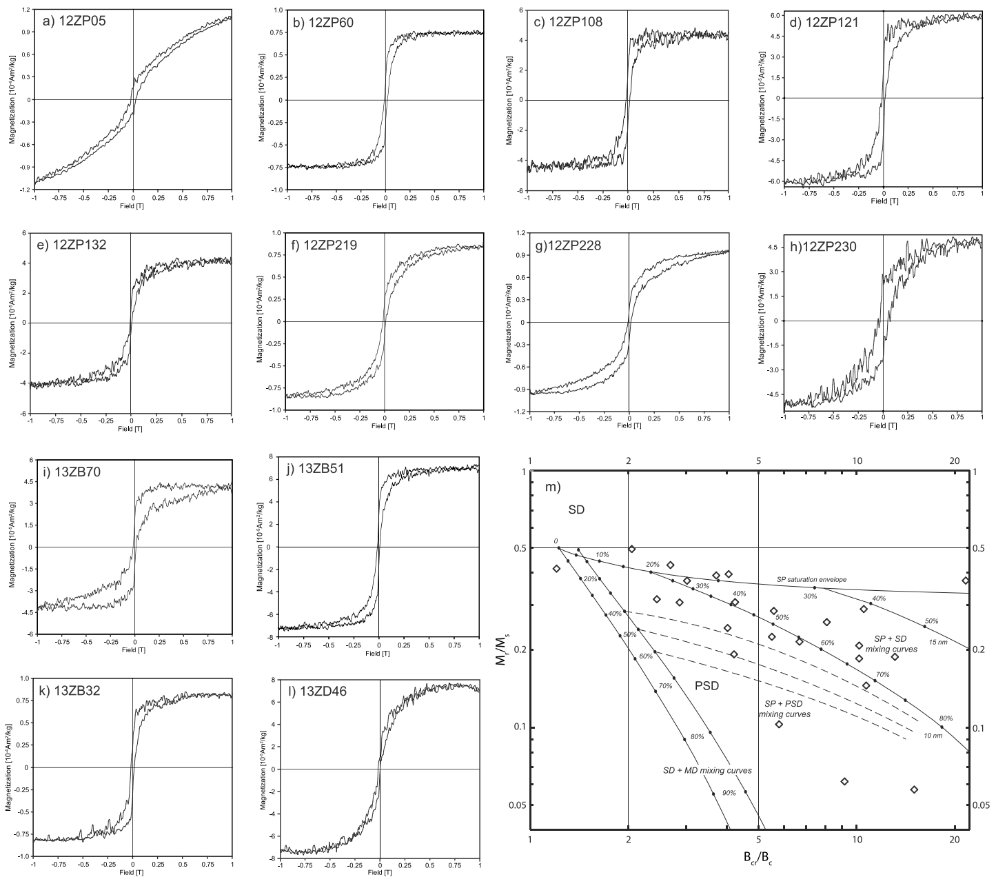
Figure 4. (a–l) Room temperature hysteresis loops from representative specimens of the Zongpu carbonate rocks. (m) Day plot [Dunlop, 2002] of the hysteresis parameters for Zongpu carbonate rocks.
