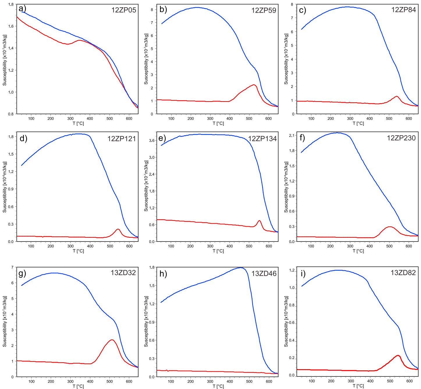
Figure 3. High-temperature heating (red) and cooling curves (blue) of bulk magnetic susceptibility in air for representative specimens.
